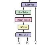
Scaled Dot-Product Attention
